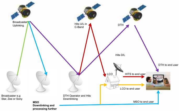
FIG. 1: Transmission of TV signal from Broadcaster to Subscriber
